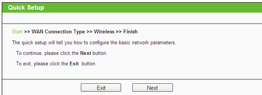
Figure 3-5 Quick Setup
