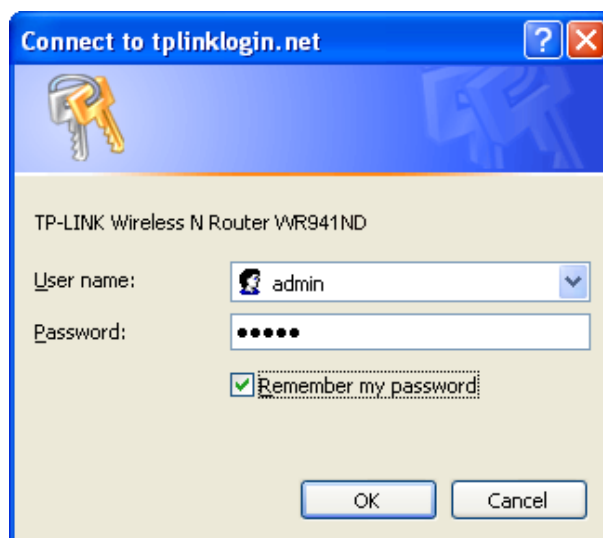
Figure 3-4 Login Windows
