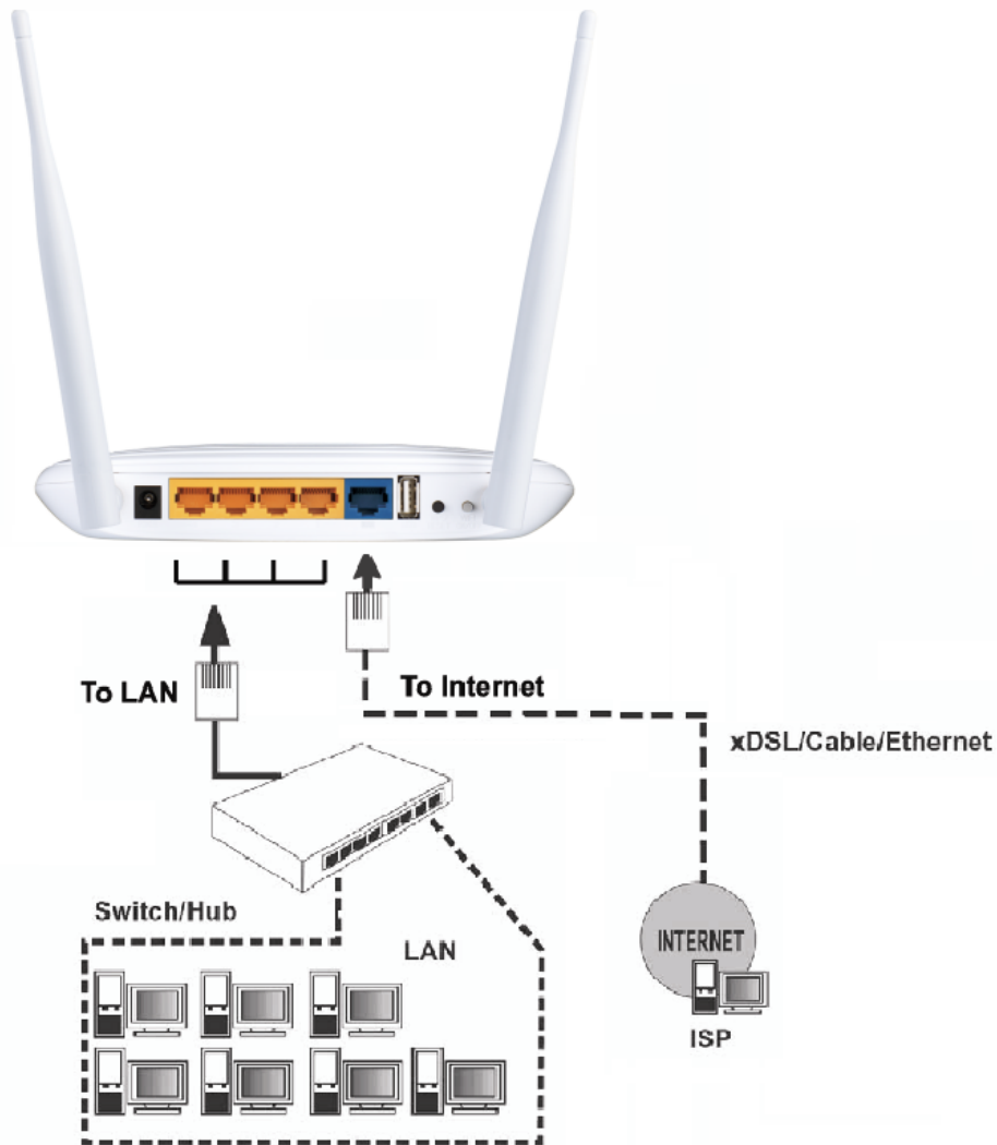
Figure 2-1 Hardware Installation
