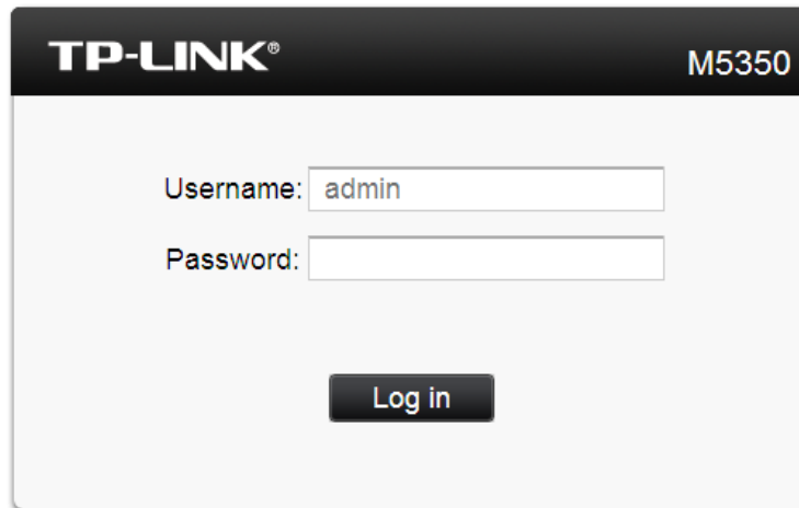
Figure 3-1 Login Window
