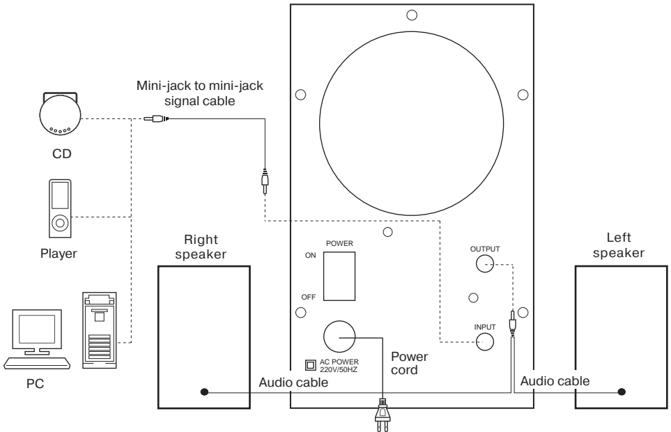
Fig. 3. Connection diagram
