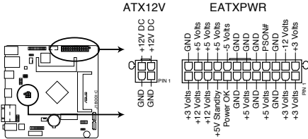
J1800I-C ATX power connectors
