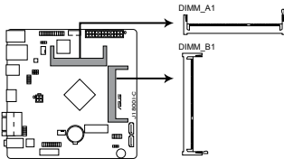
J1800I-C 204-pin DDR3 SO-DIMM sockets
