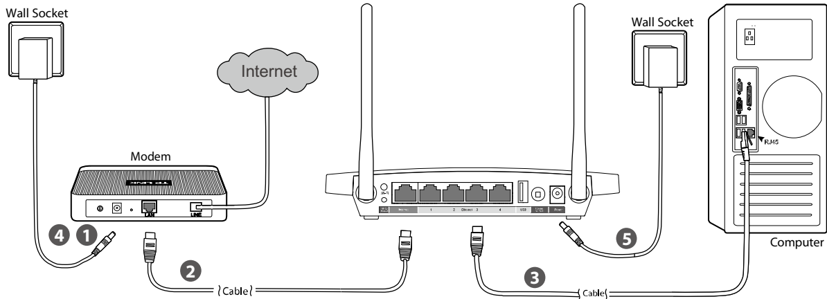
Figure 2-1 Hardware Installation
