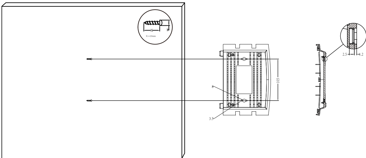
Figure 2-2 Wall-mount Installation
